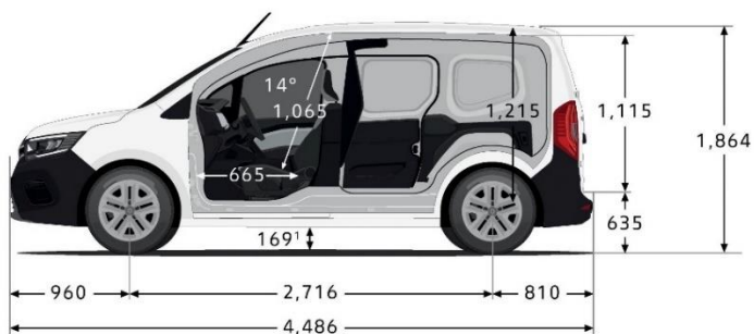
Dimensions (mm)
